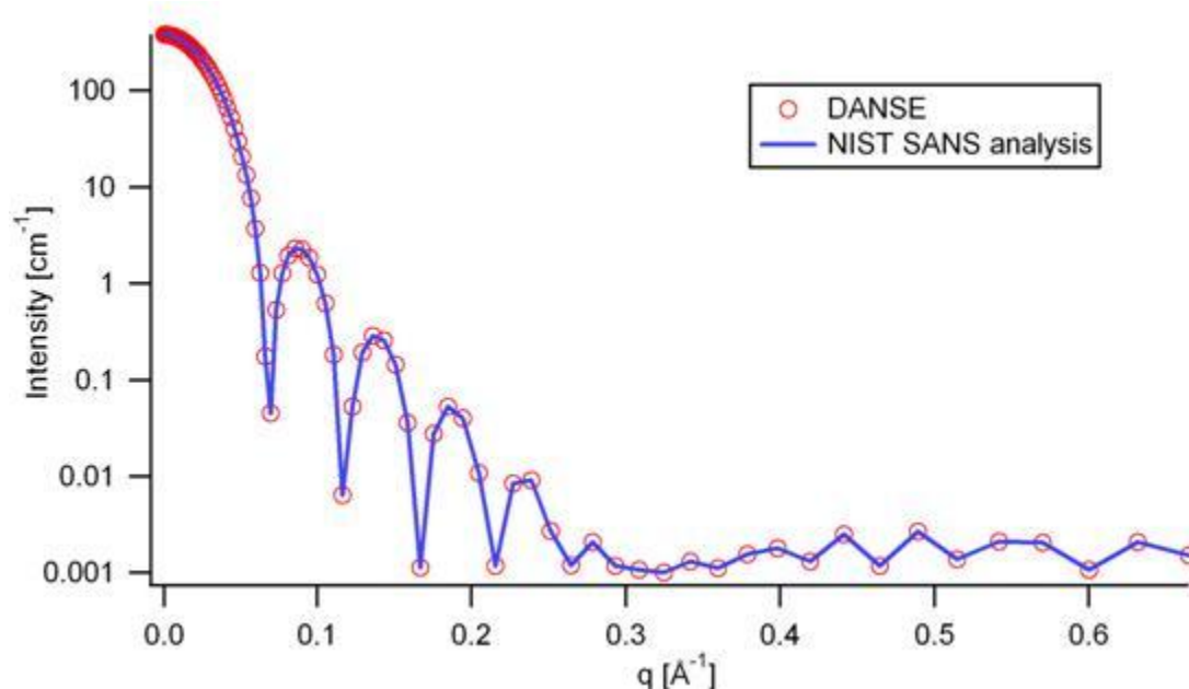
Figure 7: Comparison of the DANSE scattering intensity for a core-shell sphere with the output of the NIST SANS analysis software. The parameters were set to: Scale=1.0, Radius=60 \text{\AA} , Contrast=1e-6 \text{\AA}^{-2} , and Background=0.001 \text{cm}^{-1} .
